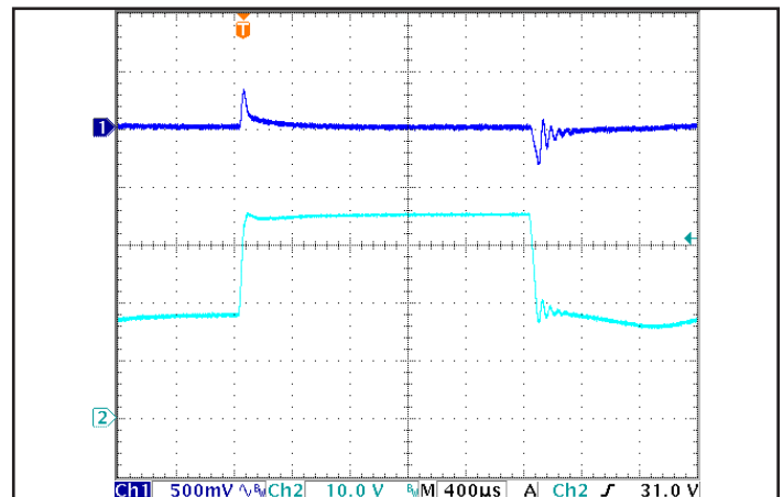
Figure 6: Output voltage response to step-change in input voltage (1000 V/ms). Load cap: 100 \mu F , electrolytic output capacitance. Ch 1: V_{out} (500 mV/div), Ch 2: V_{in} (10 V/div).
