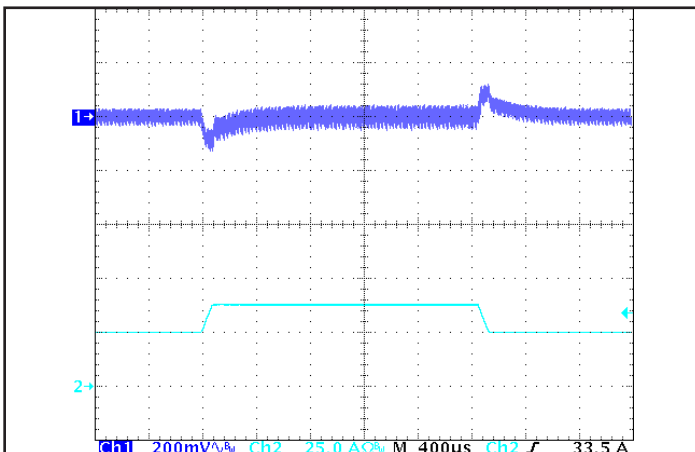
Figure 5: Output voltage response to step-change in load current (66% -100% -66% of I out (max); dI/dt = 0.1 A/μs). Load cap: 1 μF ceramic capacitor. Ch 1: V out (200 mV/div), Ch 2: I out (25 A/div).
