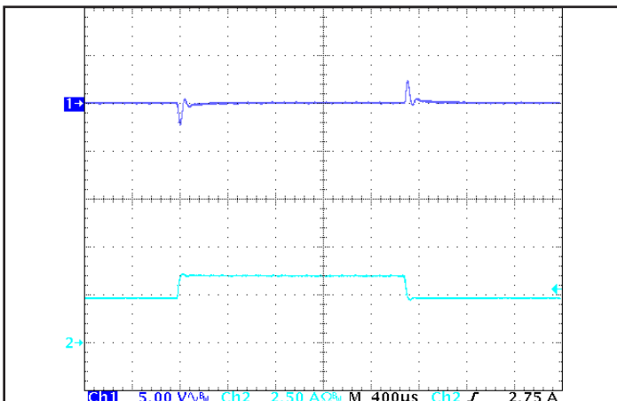
Figure 5: Output voltage response to step-change in load current (66% -100% -66% of I out (max); dI/dt = 0.02 A/μs). Load cap: 1 μF ceramic capacitor. Ch 1: V out (5 V/div), Ch 2: I out (2.5 A/div).
