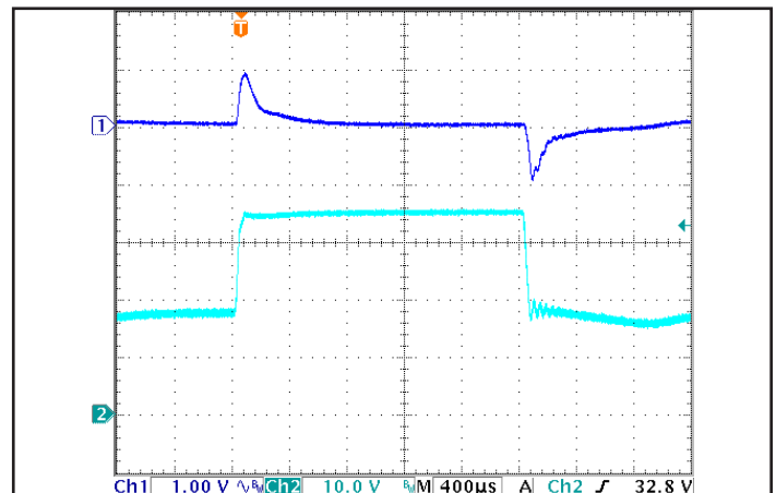
Figure 6: Output voltage response to step-change in input voltage (500 V/ms). Load cap: 100 \mu F , electrolytic output capacitance. Ch 1: V_{out} (1 V/div), Ch 2: V_{in} (10 V/div).
