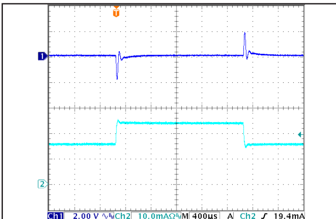
Figure 5: Output voltage response to step-change in load current (66% -100% -66% of I out (max); dI/dt = 0.1 A/μs). Load cap: 1 μF ceramic capacitor. Ch 1: V out (2 V/div), Ch 2: I out (2 A/div).
