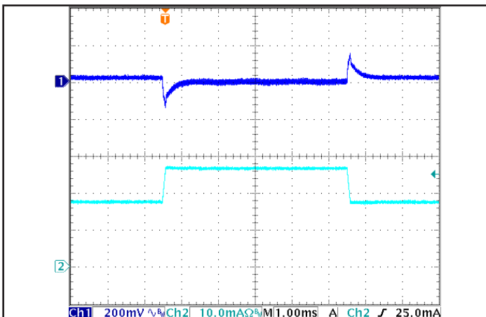
Figure 5: Output voltage response to step-change in load current (66% -100% -66% of I_{out(max)} ; dI/dt = 0.1 A/\mu s ). Load cap: 1 \mu F ceramic capacitor. Ch 1: V_{out} (200 mV/div), Ch 2: I_{out} (10 A/div).
